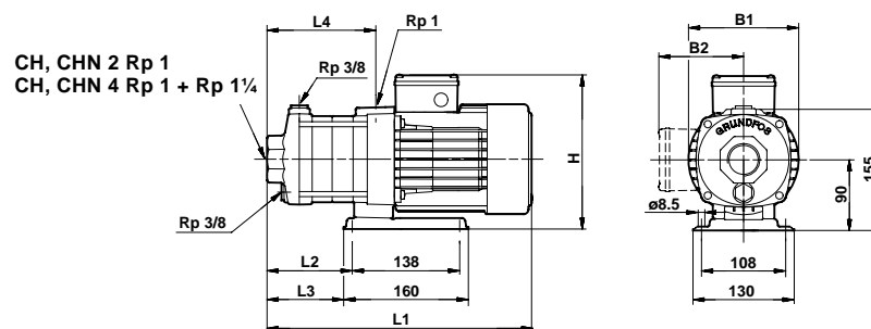
Fig. 5 Dimensional sketches, CH, CHN 2 and 4 with MG 71/80 motor
